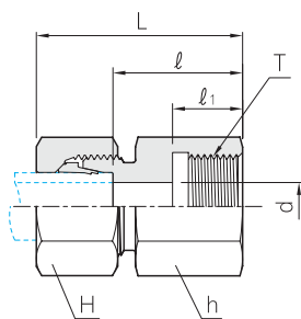
Form Y Tapped Hole
